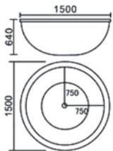
SWP-BT-007 Size : 1500 x 1500 x 640mm
