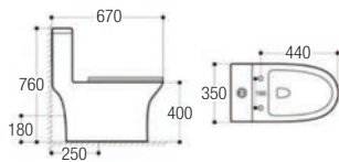
WC-9393-S250-G (GOLD) Washdown One-Piece Closet Size : 670 x 350 x 760mm S-Trap : 250mm Roughing-In Quantity : 1 set /c tn
