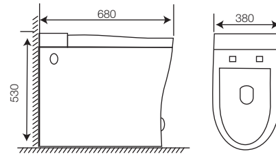
WC-1004/WC-1005 (I-Voice) Intelligent Water Closet
