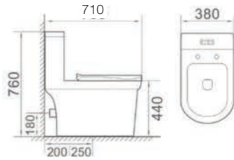
WC-2090-Black Washdown One-Piece Closet - Black Size: 710 x 380 x 760mm S-trap-250mm Roughing-in Quantity : 1 set/ctn
