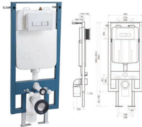
SWACC-006 Front Push Concealed Cistern With Frame & Pipe Set
