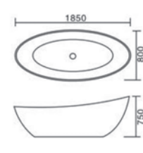
SWP-BT-1056 Size : 1850 x 800 x 750mm
