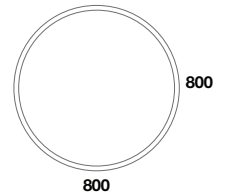
SWMR-8080-BK Black Aluminium Frame Round Frame Mirror c/w Shelf Mirror Size : 800mmx800mm Shelf Size : Without Shelf Quantity : 1set/box | 1set/ctn
